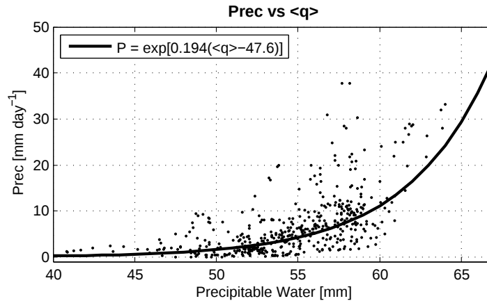
Figure 3.3: Precipitation as a function of precipitable water \langle q \rangle . The black line was computed by a nonlinear least squares fitting.
