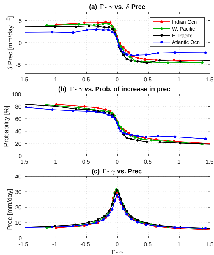
Figure 4.5: As in Fig. 4.3, but the critical GMS \Gamma_C was replaced with the slopes of the regression lines \gamma in the left panels of Fig. 4.4.
