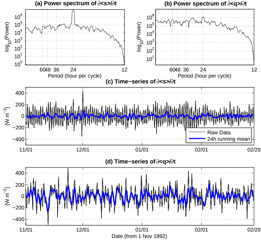
Figure 3.2: (a): Power spectrum of \partial\langle s \rangle / \partial t . (b): Power spectrum of \partial\langle q \rangle / \partial t . (c): Time-series of raw (black), and daily running averaged \partial\langle s \rangle / \partial t (blue) during TOGA COARE. (d): As in (c), but for \partial\langle q \rangle / \partial t . The mixing ratio q is scaled by the latent heat of evaporation into the energy unit.
