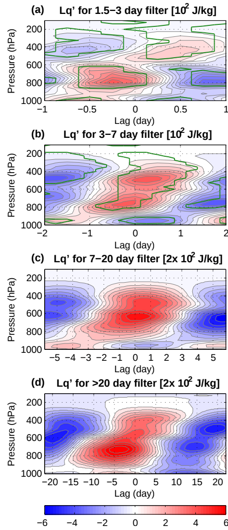
Figure 2.7: As in Fig. 2.3, but for anomalous mixing ratio. The contour intervals are 0.6 \times 10^2 J/kg for (a) \sim 2 day, (b) \sim 5 day scales, and 1.2 \times 10^2 J/kg for (c) \sim 10 day and (d) the MJO scales.
