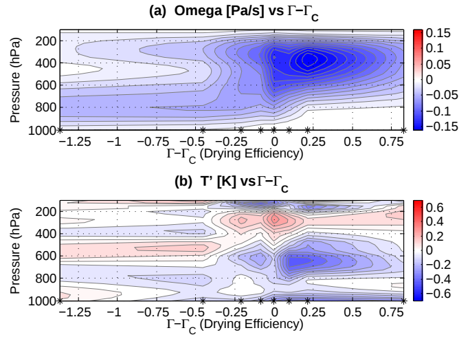
Figure 3.9: (a): Binned vertical \omega structures with respect to the drying efficiency \Gamma - \Gamma_c for convectively active times ( \nabla \cdot \langle s \mathbf{v} \rangle > 0 ), averaged in the same bins as in Figs. 3.4 and 3.5. The star-marks on the x-axis denote the bin-centers. The contour interval is 2 \cdot 10^{-2} Pa/s. (b): As in (a), but for temperature anomalies. The contour interval is 0.1 K.
