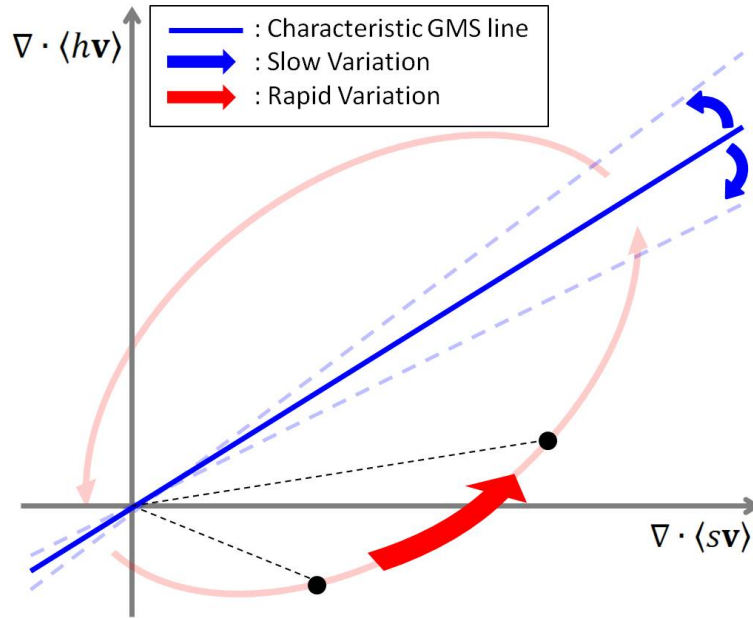
Figure 3.14: Schematic figure of a convective life-cycle (light-red arrows) in the \nabla \cdot \langle h\mathbf{v} \rangle -vs- \nabla \cdot \langle s\mathbf{v} \rangle plane. The thick red arrow represents variation of highly time-dependent GMS; the blue thick arrows represent variation of slowly changing climatological GMS.
