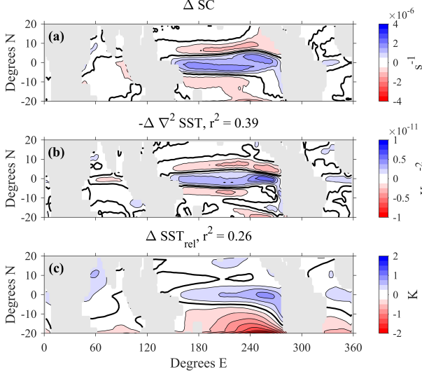
FIG. 4. Ensemble-mean response to climate change of (a) SC (contour interval: 5 \times 10^{-7} \text{ s}^{-1} ), (b) negative of \nabla^2 \text{SST} (smoothed, contour interval: 1.25 \times 10^{-12} \text{ K m}^{-2} ), and (c) \text{SST}_{\text{rel}} (contour interval: 0.25 K). Zero contour denoted by thick black contour. Values of r^2 in (b) and (c) are for monthly climatological values relative to the change in SC from the GCMs.
