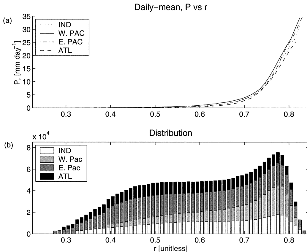
FIG. 3. (a) Mean daily averaged precipitation P in 1% bins of column-relative humidity r , for the four tropical ocean regions in Fig. 1 for all months in 1998–2001. (b) Number of observations in each bin in the four regions.
