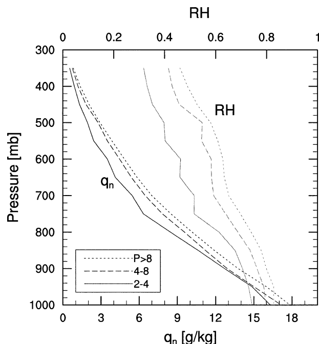
FIG. 9. Radiosonde-derived profiles of normalized monthly mean specific humidity ( W^{\text{ref}}/W_* ) q (left curves) and relative humidity (right curves), bin averaged by monthly mean Xie–Arkin precipitation ( \text{mm day}^{-1} ). The profiles are derived from Jan, Apr, Jul, and Oct climatologies at the 24 long-term radiosonde sites in 20^\circ\text{S} – 20^\circ\text{N} shown in Fig. 1.
